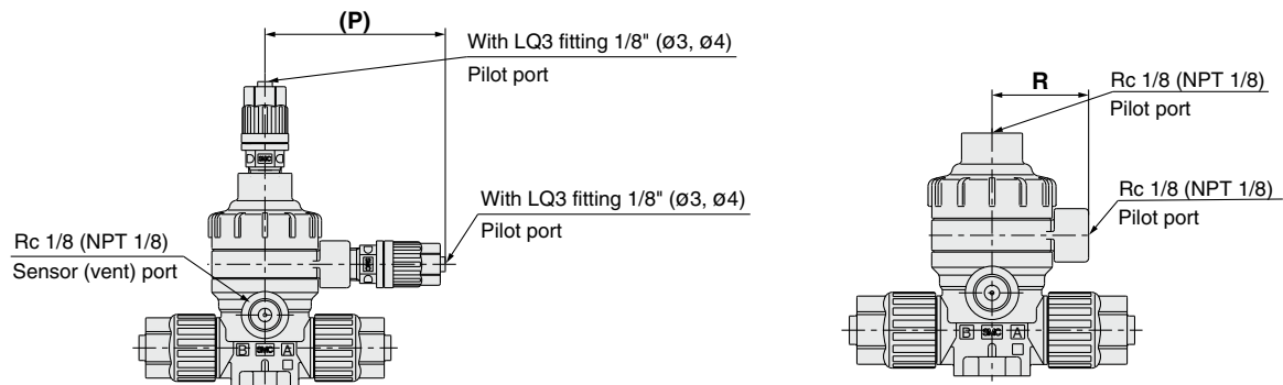
LVQ \square_2 -Z \square\square Dimensions (N.O. Valve, Double Acting Valve)
