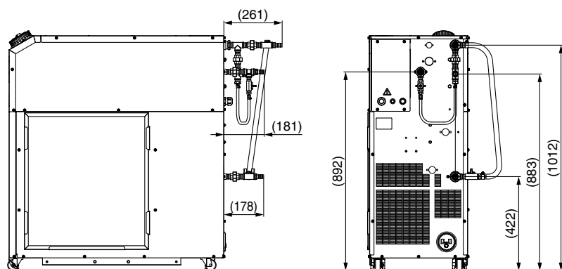
Mounting dimensions: HRLE050
