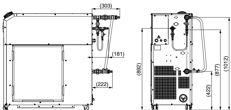
Mounting dimensions: HRLE090
