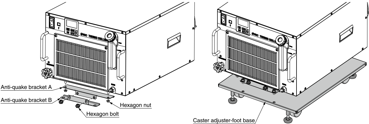
Mounting view
