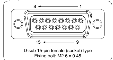
Contact input/output signal connector
