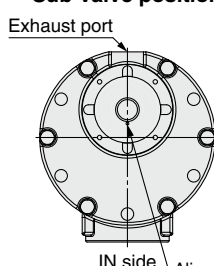
Fig. 1 Valve position
