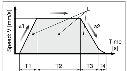
<Speed-Work Load Graph> (LEKFS40)
