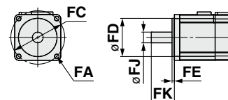
Applicable motor dimensions
