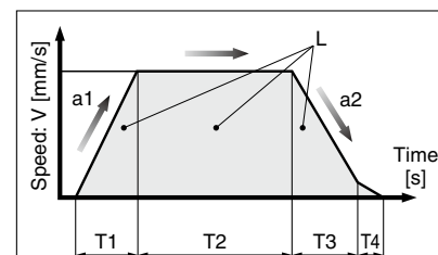
<Speed-Work Load Graph> (LEFB40)
