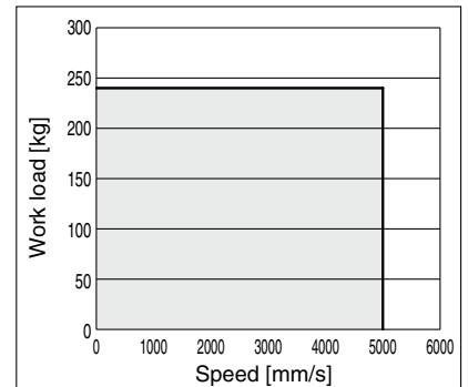
<Speed-Work Load Graph> (LET100)
