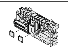
EXH block plate VVQ2000-19A
